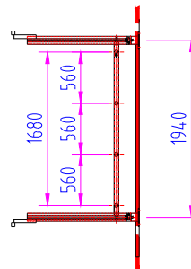
Kletterstange
